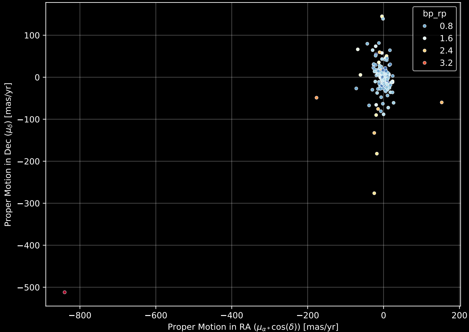
APOGEE DR17 Field: [090+34_MGA] Proper Motion Diagram (n= 203)
