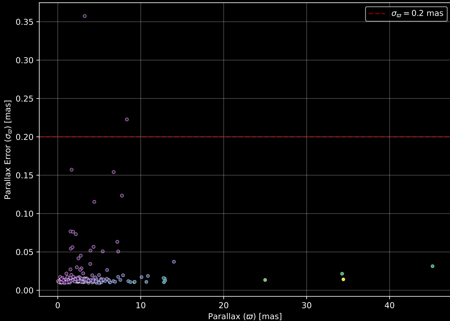
APOGEE DR17 Field: [090+34_MGA] Parallax Quality (n= 203)
