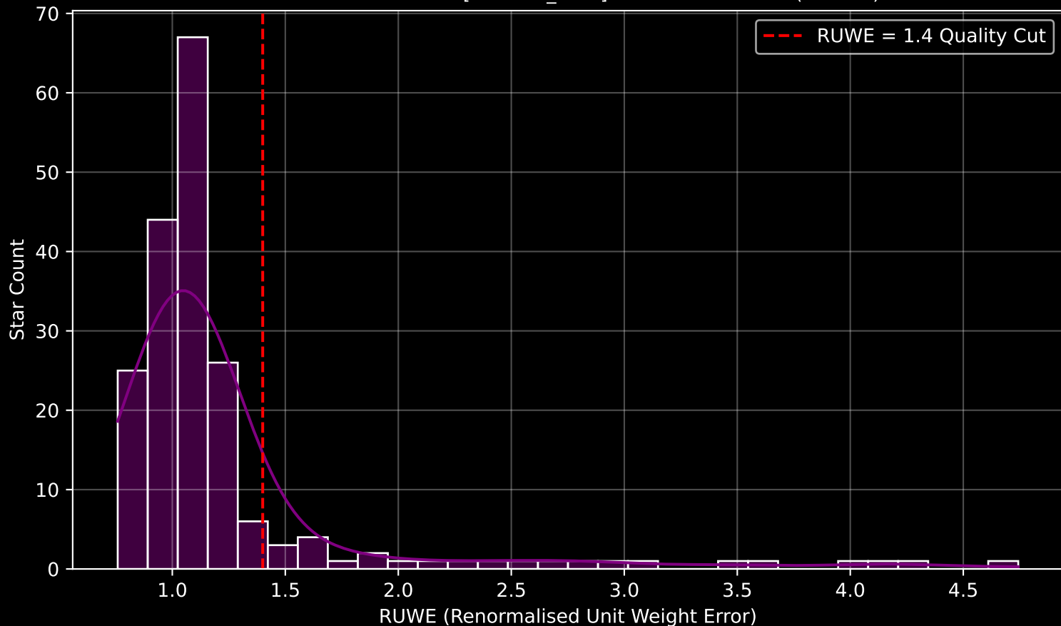
GAPOGEE DR17 Field [090+34_MGA] RUWE Distribution (n= 193)
