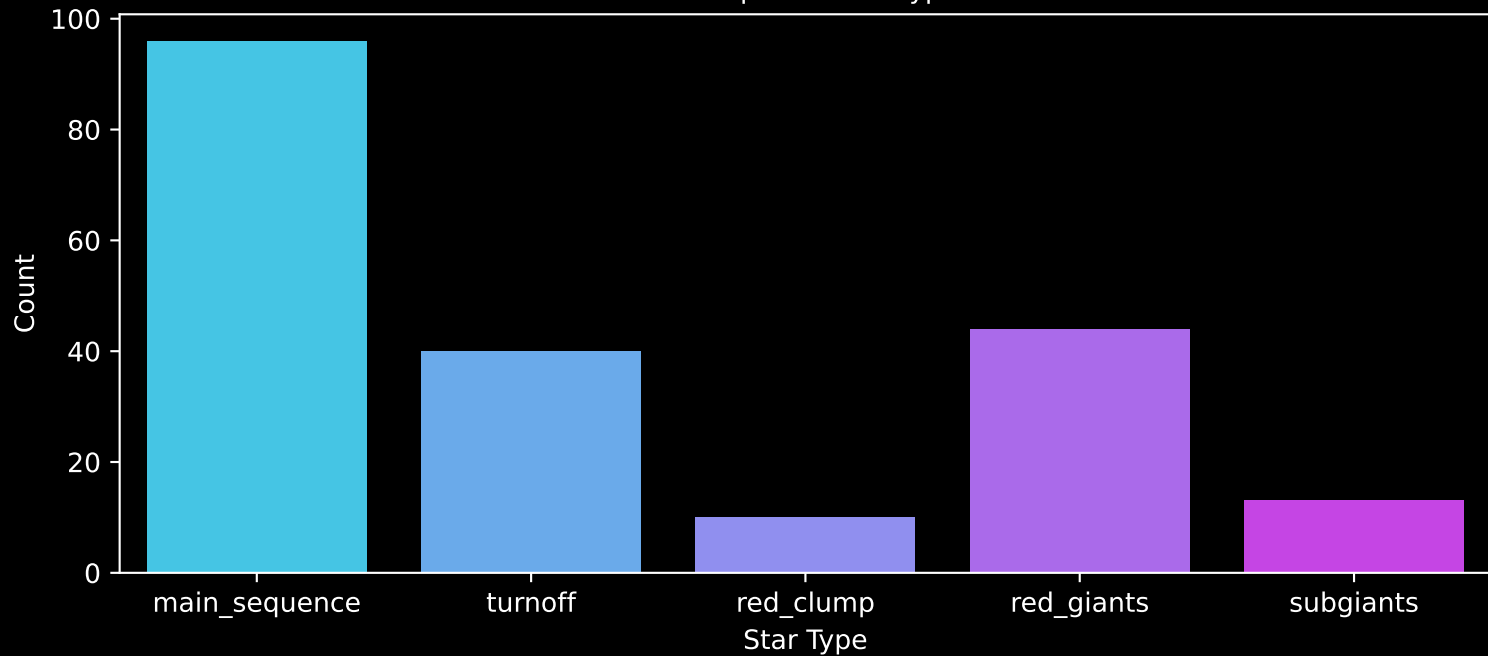
APOGEE DR17 Field: [090+34_MGA] Count plot of Star Type
