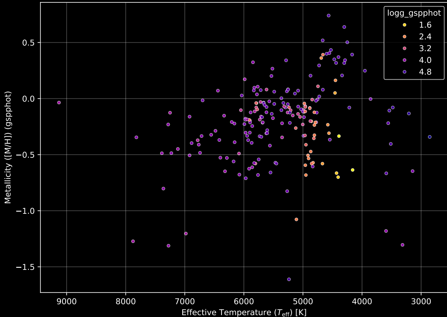
APOGEE DR17 Field: [090+34_MGA] Stellar Population Parameters (n= 203)
