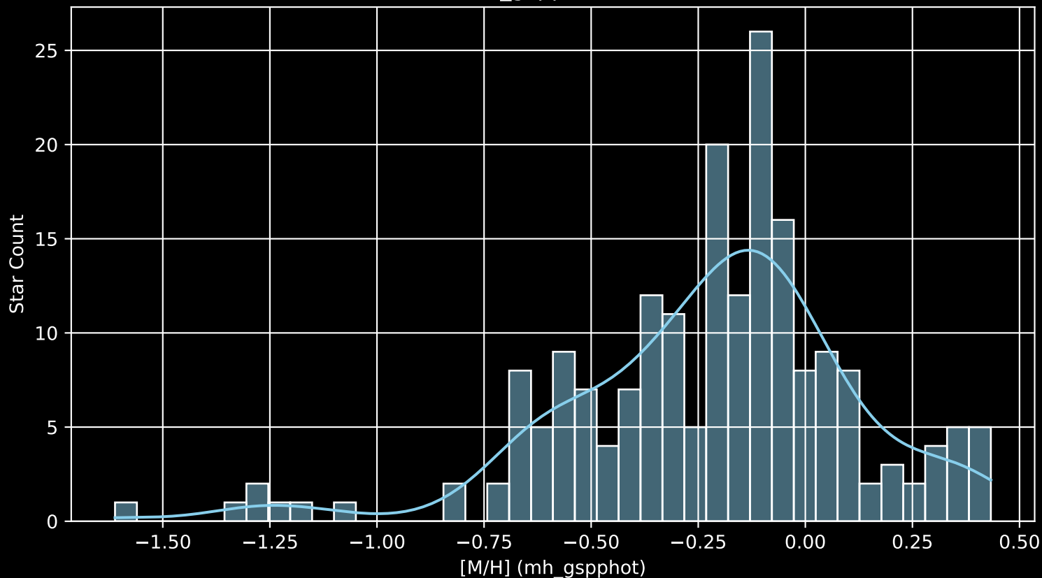
APOGEE DR17 Field: [090+34_MGA [M/H] (mh_gspphot) (n= 199)
